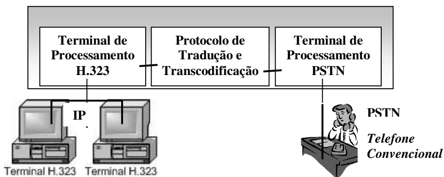
Figura 8: Gateway H.323/PSTN.
