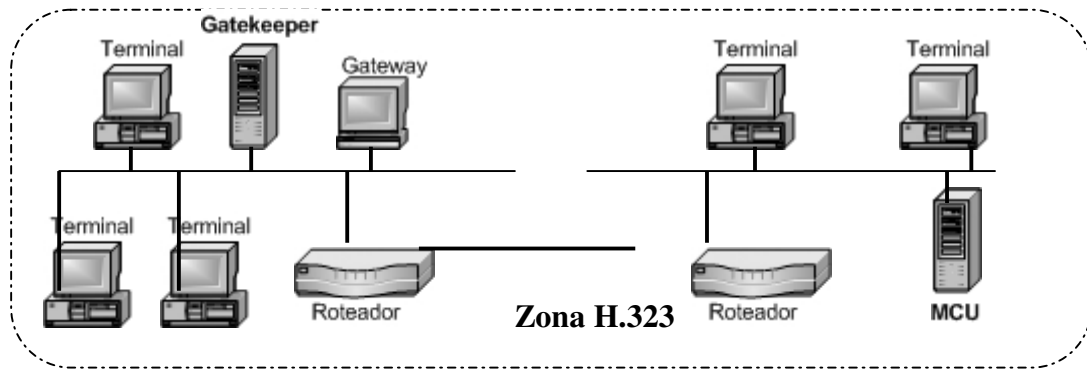
Figura 9: Gatekeeper H.323.
