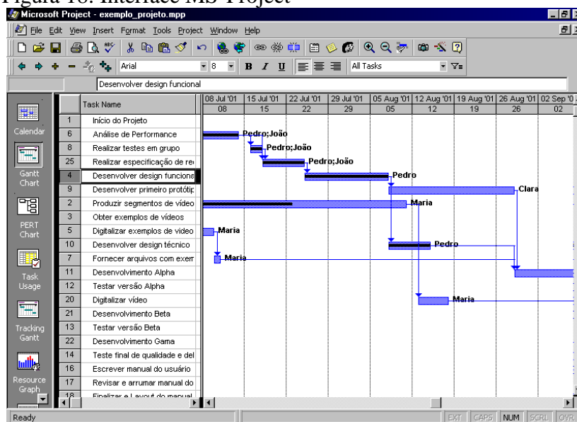
Figura 18: Interface MS-Project
