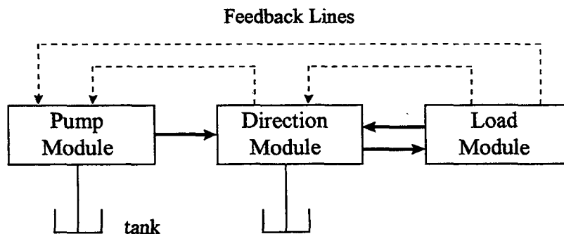
Figure 4.1- Typical modules for a hydraulic system (SARGENT et al., 88)
