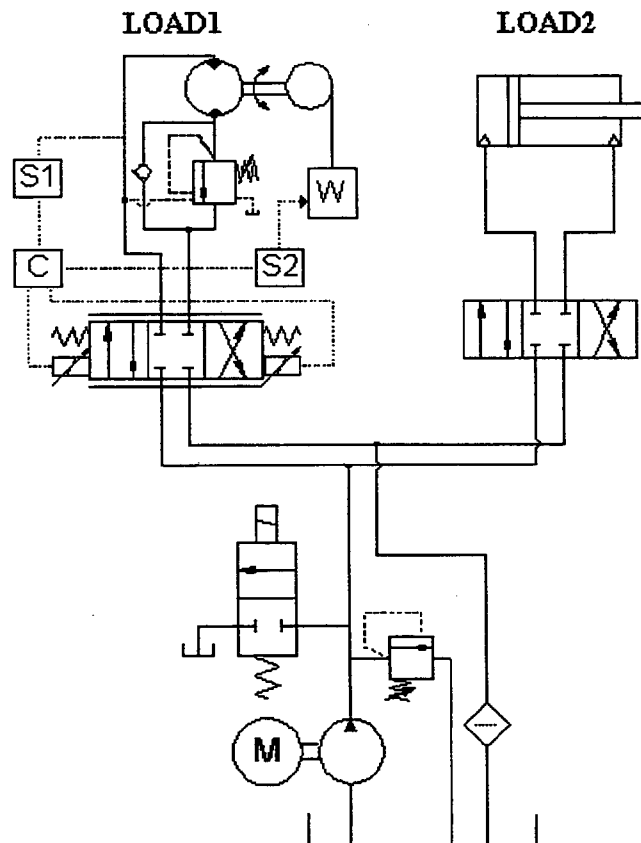
Figure A2.1- Hydraulic system diagram for the first problem.
