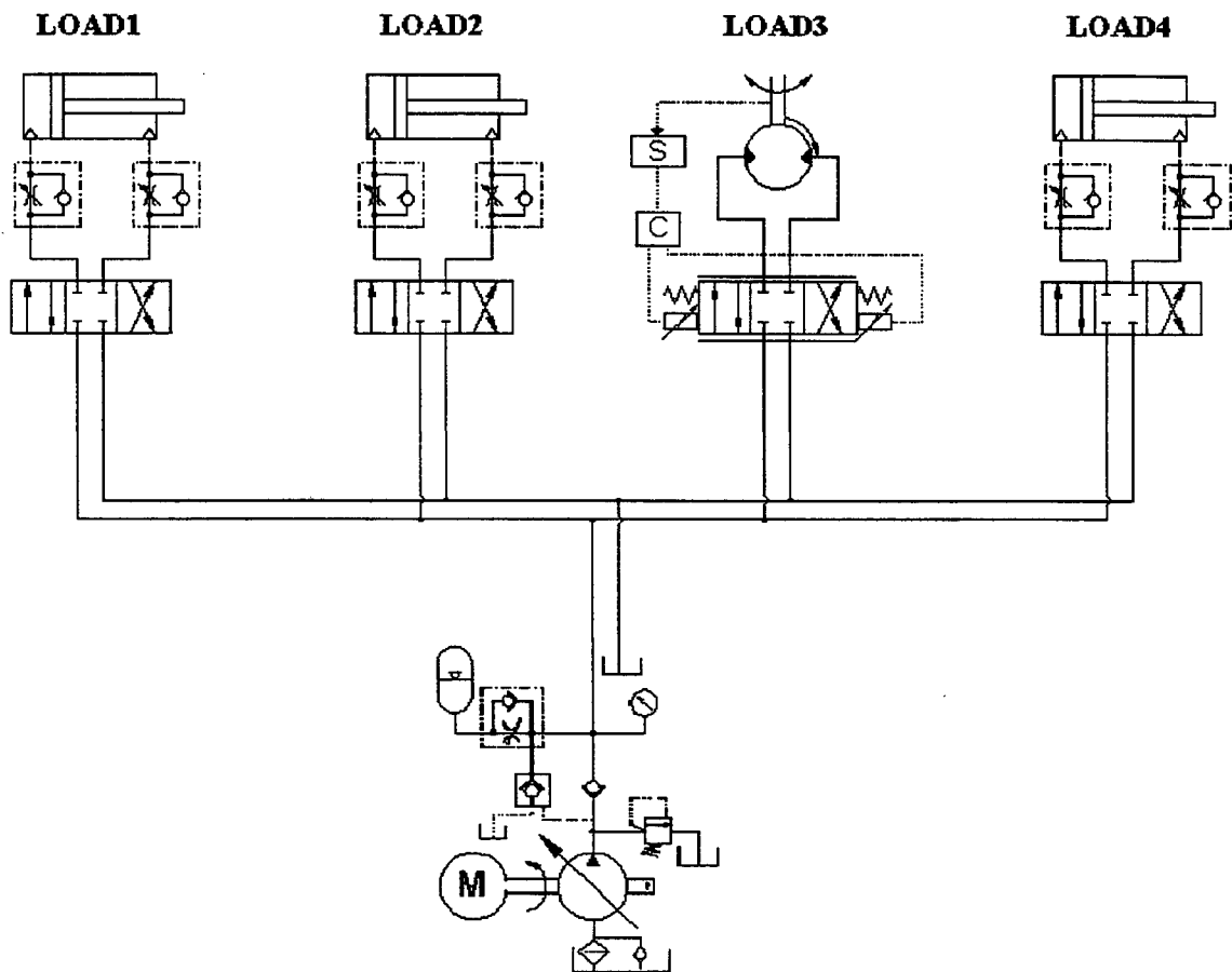
Figure A2.5- One alternative system diagram for a moulding machine.
