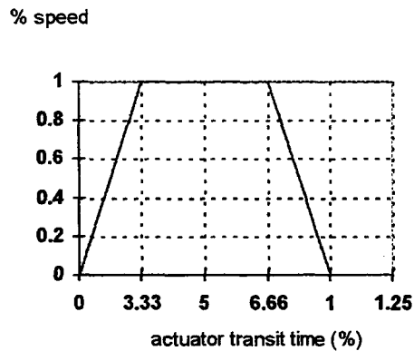
Figure 4.5. Trapezoidal Speed Profile (CLEASBY,96).
