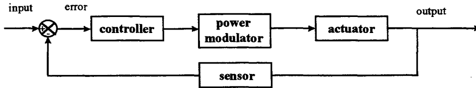
Figure 4.4. General Servo System Structure.
