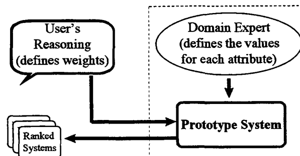
Figure 5.15- Ranking process.
