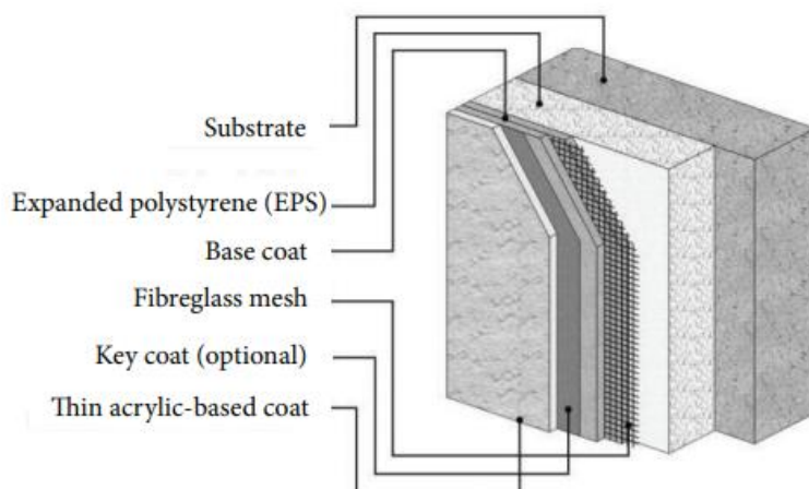
Figure 1: Schematic example of ETICS available in the Portuguese market. Source: BARREIRA; FREITAS (2014), FREITAS (2002).
