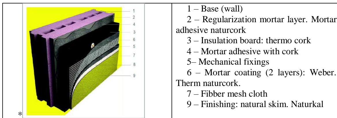
Figure 2: Composition of insulating coating for exterior (ETICs). Fonte: Weber Naturcork (2020).
