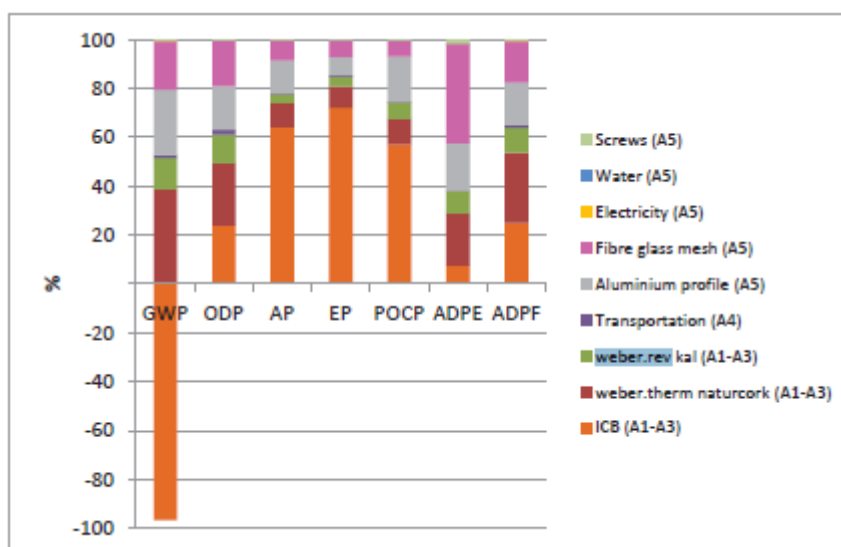
Figure 5: Comparative of Impact characterisation of mortar lime (green color) with another components of the ETICS. Source: Weber; Centro Habitat Portugal (2020).
