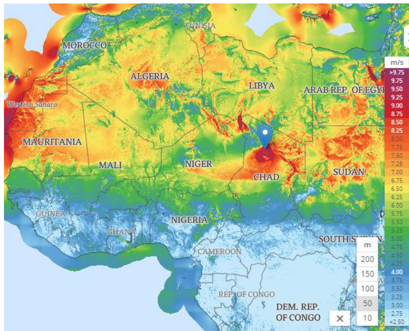
Figure 7: Incidence of winds at 50 meters. Signaling made by the authors. Fonte: Global Wind Atlas (2019)
