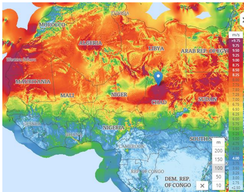
Figure 8: Incidence of winds at 100 meters. Signaling made by the authors. Fonte: Global Wind Atlas (2019)
