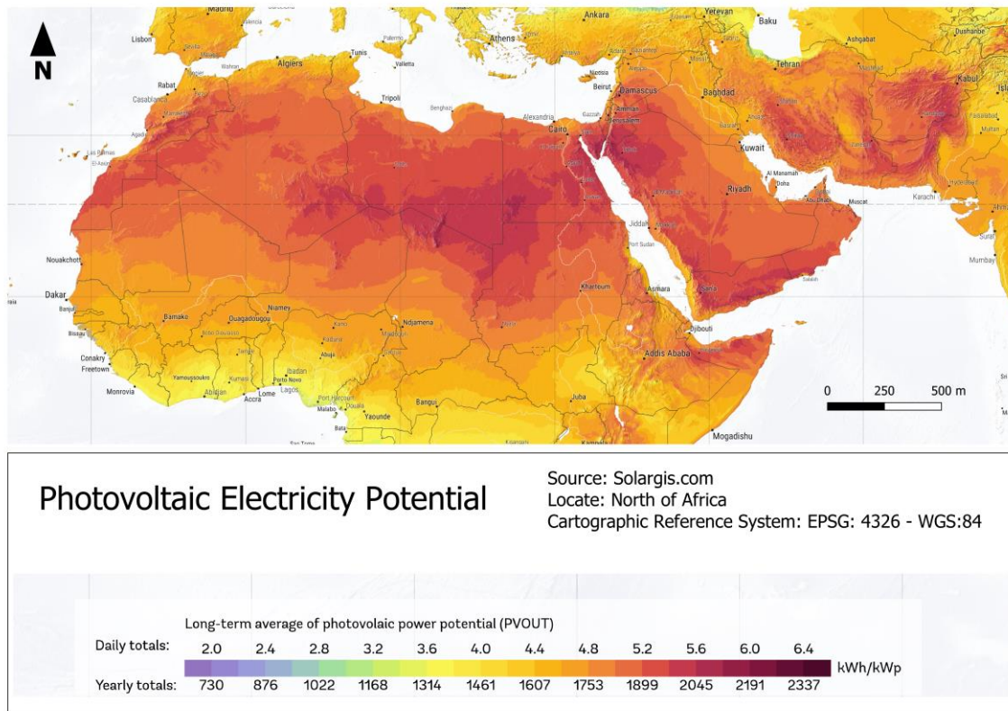
Figure 6: Photovoltaic Electricity Potential. Source: Elaborated by the authors
