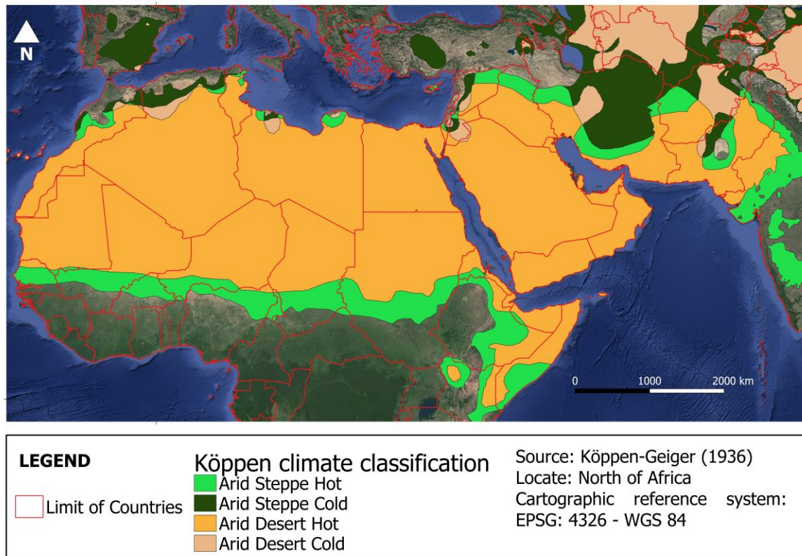
Figure 3: Köppen-Geiger Climate Classification. Source: Elaborated by the authors
