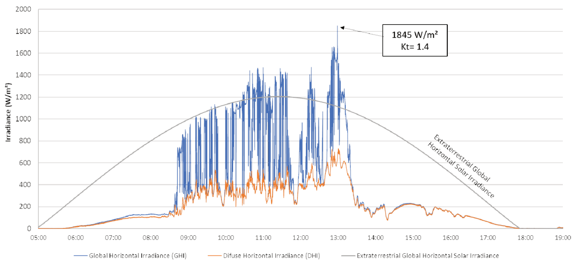
Figure 37 - Highest overirradiance event measured in Brazil so far (1845 W/m 2 ), using a Delta SPN1 thermopile pyranometer installed at the # Caucaia-CE SMS.
