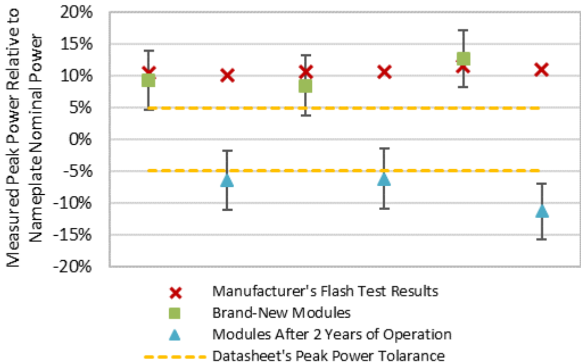
Figure 32 - I-V curve measurement results of three brand-new 142 Wp a-Si/ \mu c-Si PV modules (green squares), and three 142 Wp a-Si/ \mu c-Si PV modules that had been operating in the ES for two years (blue triangles). The flash test results provided by the manufacturer for these specific six modules are also shown as red Xs. The tolerance indicated by the manufacturer on the PV module's datasheet is shown as yellow dashed lines.
