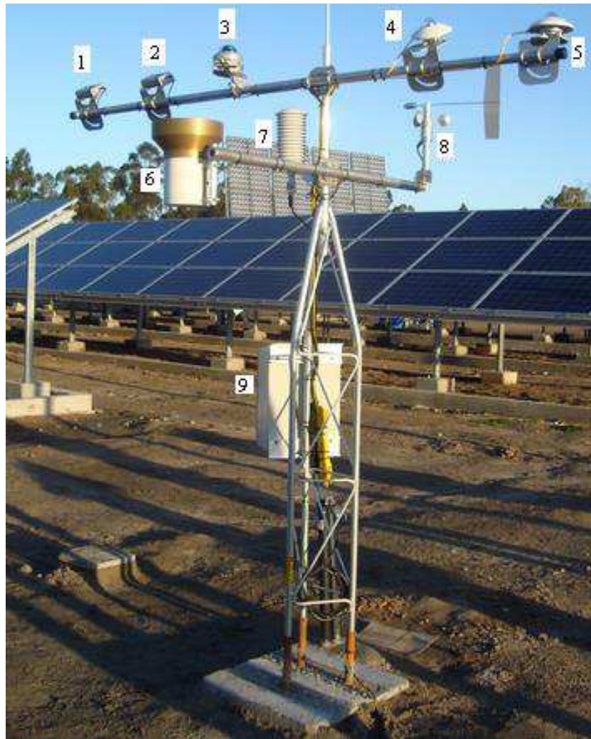
Figure 25 - Solar monitoring station installed at the Capivari de Baixo-SC ES, with identical sensors installed in all eight ESs and detailed in Table 5.
