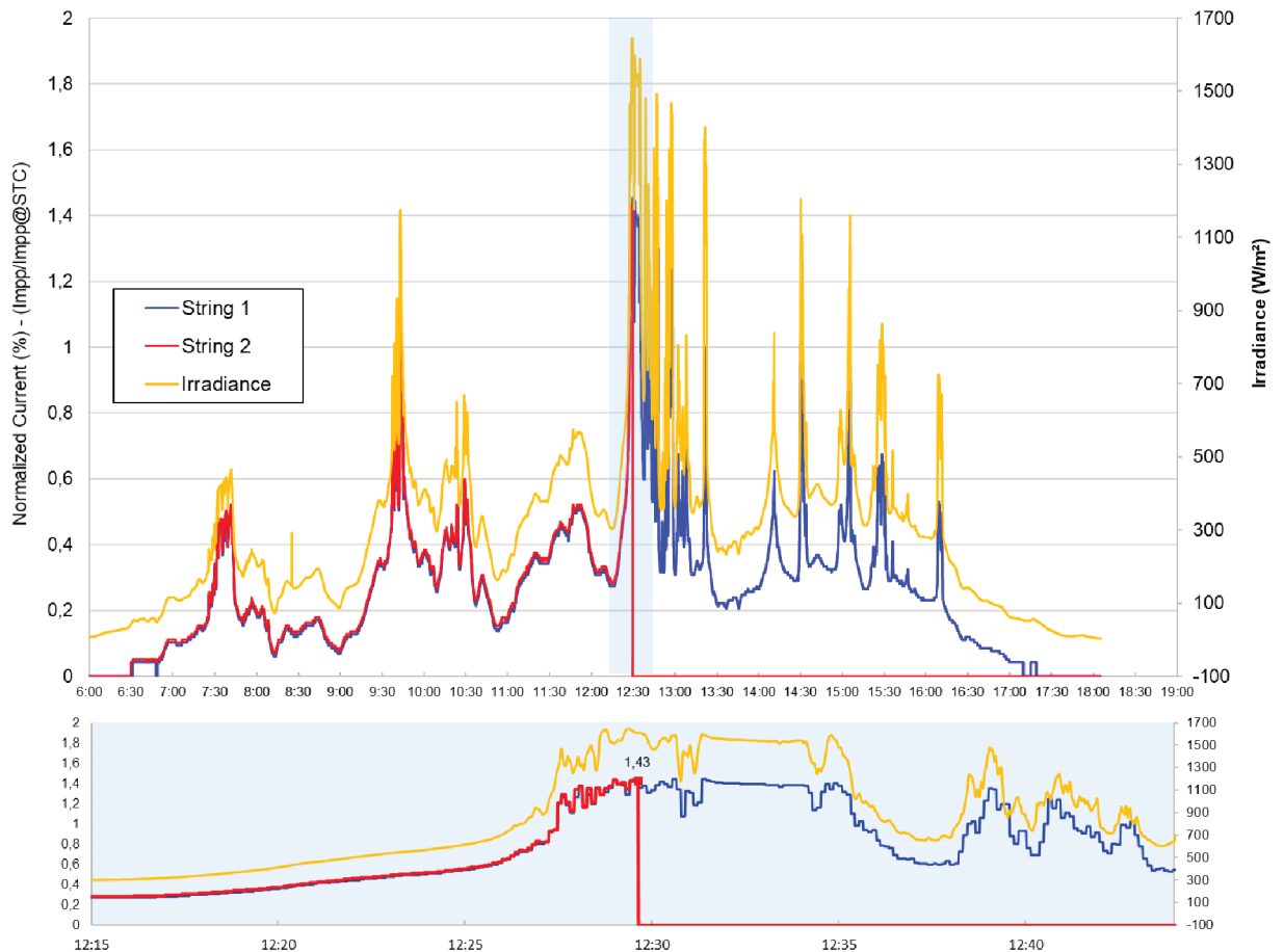
Figure 42 - Global tilted overirradiance event measured with a Kipp & Zonen CMP11 thermopile pyranometer at the # Cabo Frio-RJ SMS, around 12:30, with irradiances higher than 1500 \text{ W/m}^2 and lasting longer than five minutes. The fuse of string 2 has blown with a normalized current value of 1.43.
