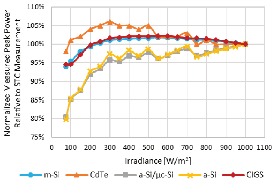
Figure 33 - Weak-light response of brand-new PV modules of five technologies identical to the ones employed at the ESs. Measurements were made in a PASAN SunSim3CLAPSS AAA solar simulator, at LABSOL-UFRGS, and corrected to STC. Results are shown in relation to each technology's STC measurement.
