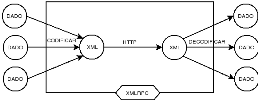
Figura 3: Protocolo XML-RPC [WINER, 1999]
