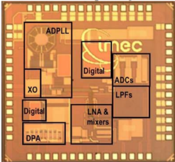
Figura 15 – F-Integrated RF IEEE 802.11ah
