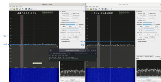
Figure 9: Reception using gqrx for 50 degrees LOS condition. Right: Gqrx with reception from setup with filter and in Left: Gqrx with reception from setup without filter.
