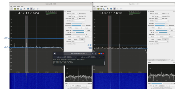
Figure 8: Reception using gqrx for 72 degrees TCA condition. Right: Gqrx with reception from setup with filter and in Left: Gqrx with reception from setup without filter.
