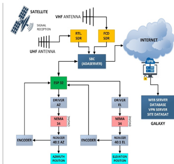
Figure 3: Operational Diagram of the ADA equipment.
