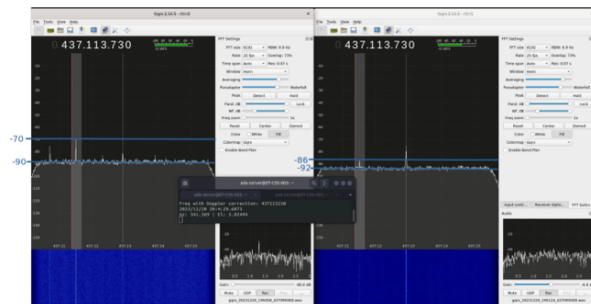
Figure 10: Reception using gqr for 20 degrees LOS condition. Right: Gqr with reception from setup with filter and in Left: Gqr with reception from setup without filter.
