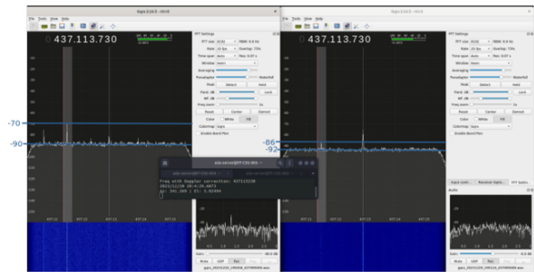
Figure 11: Reception using gqr for 5 degrees LOS condition. Right: Gqr with reception from setup with filter and in Left: Gqr with reception from setup without filter.
