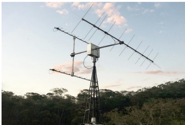
Figure 2: One of operating ADAs installed in CRIAR SPACE SYSTEMS's headquarters.
