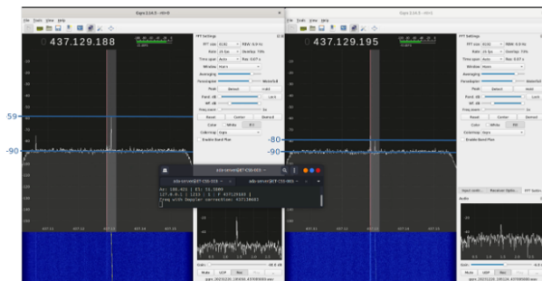
Figure 7: Reception using gqrx for 20 degrees LOS condition. Right: Gqrx with reception from setup with filter and in Left: Gqrx with reception from setup without filter.
