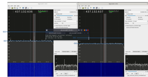
Figure 6: Reception using gqrX for 20 degrees AOS condition. Right: GqrX with reception from setup with filter and in Left: GqrX with reception from setup without filter.
